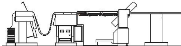
MERGER COMBO TC 7105 CUTTER TC 7722 BUFFER TC 1700 FOLDER CONVEYOR TC 0250 A
