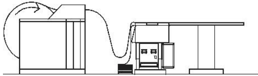
UNWINDER CUTTER TC 7712 CONVEYOR TC 0250 A
